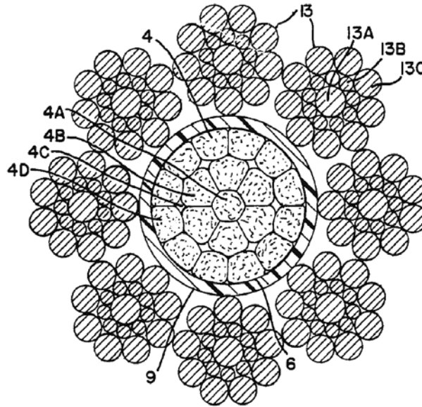
Figure 1: Composite steel wire rope as proposed by Klees et al. (1989) in their US patent filed in September 1988. 4 - Kevlar ® core and core elements, 6 - Lang's lay coated fibre core, 9 - Core protective coating, 13 - Steel outer strands.
